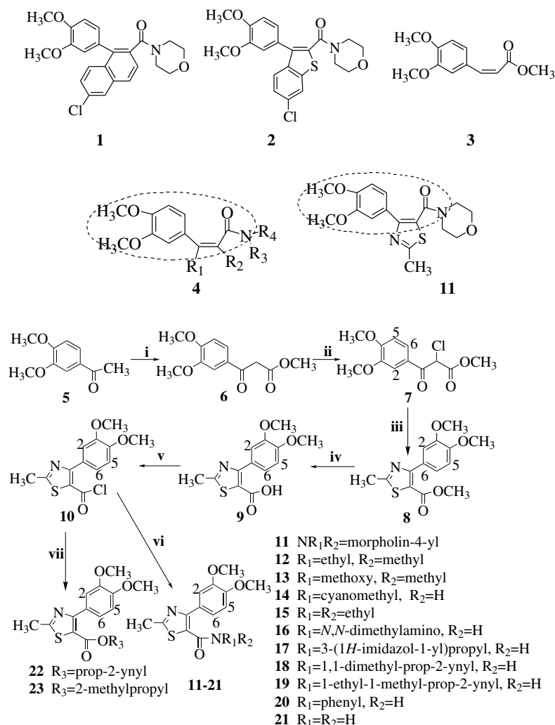
Scheme 1. Synthesis of the 4-(3,4-dimethoxyphenyl)-2-methylthiazole-5-carboxylic acid derivatives ( 11–23 ): (i) NaH/(CH 3 O) 2 CO in THF; (ii) SO 2 Cl 2 /CCl 4 ; (iii) thioacetamide/NaHCO 3 in THF; (iv) NaOH/H 2 O, HCl(aq); (v) SOCl 2 ; (vi) R 1 R 2 NH/Et 3 N in CH 3 CN; (vii) R 3 OH/Et 3 N in CH 3 CN.
