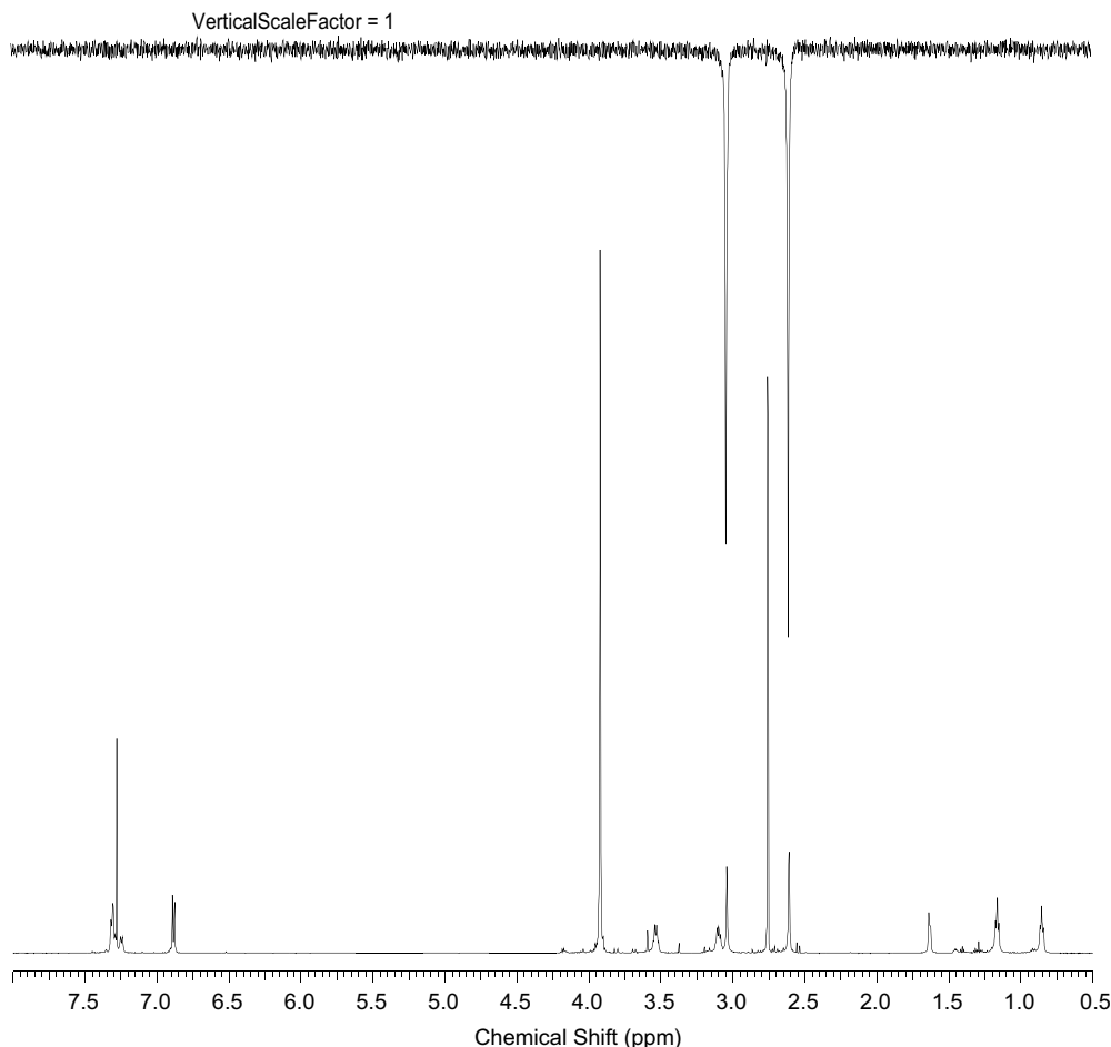
Figure 1. Saturation transfer experiment spectrum of compound 12.
